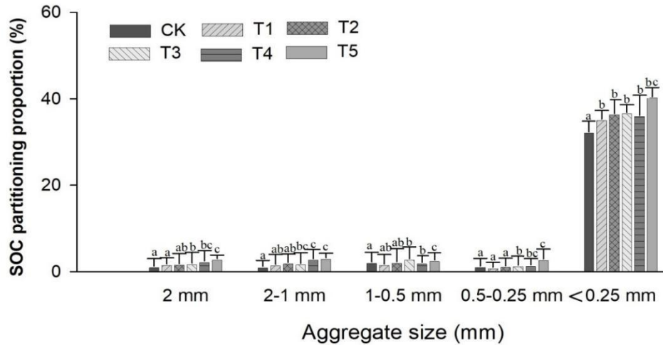
Figure 2. Partitioning proportions (%) of soil organic carbon (SOC) in water stable aggregates as influenced by biochar addition rates. Note: CK: control; T1: 4 t ha -1 , T2: 8t ha -1 , T3: 12 t ha -1 , T4: 16 t ha -1 , T5: 20 t ha -1 . Different small letters indicate significant differences as determined by the LSD test ( p \leq 0.05 ).
