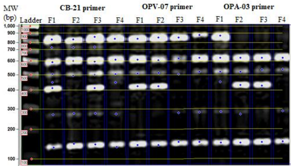
Figure S1. RAPD-PCR fingerprinting of the selected primers.
